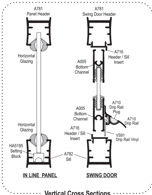
Vertical Cross Sections
