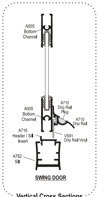
Vertical Cross Sections
