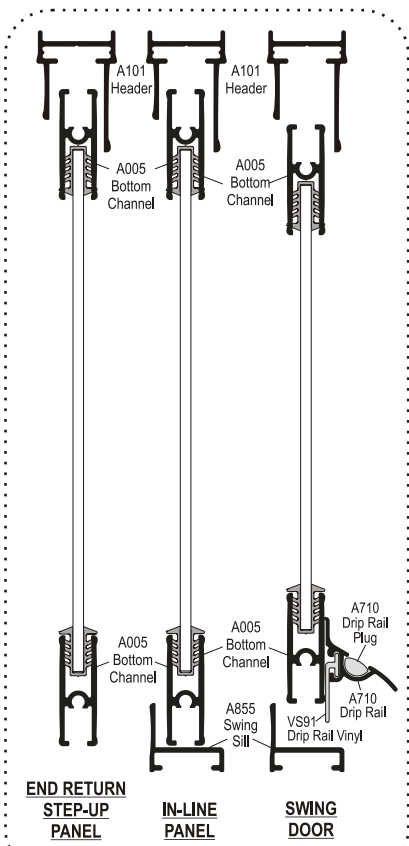
Vertical Cross Sections
