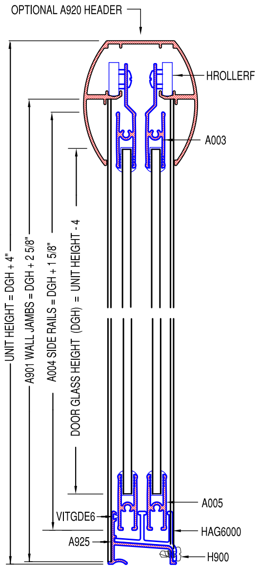
VERTICAL CROSS SECTION
