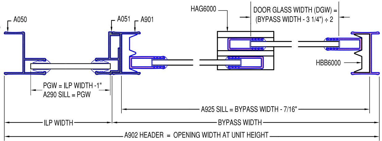
HORIZONTAL CROSS SECTION
