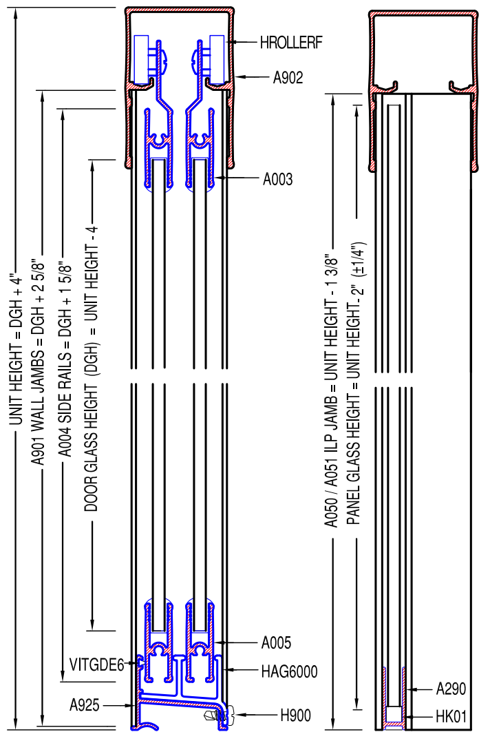
VERTICAL CROSS SECTION
