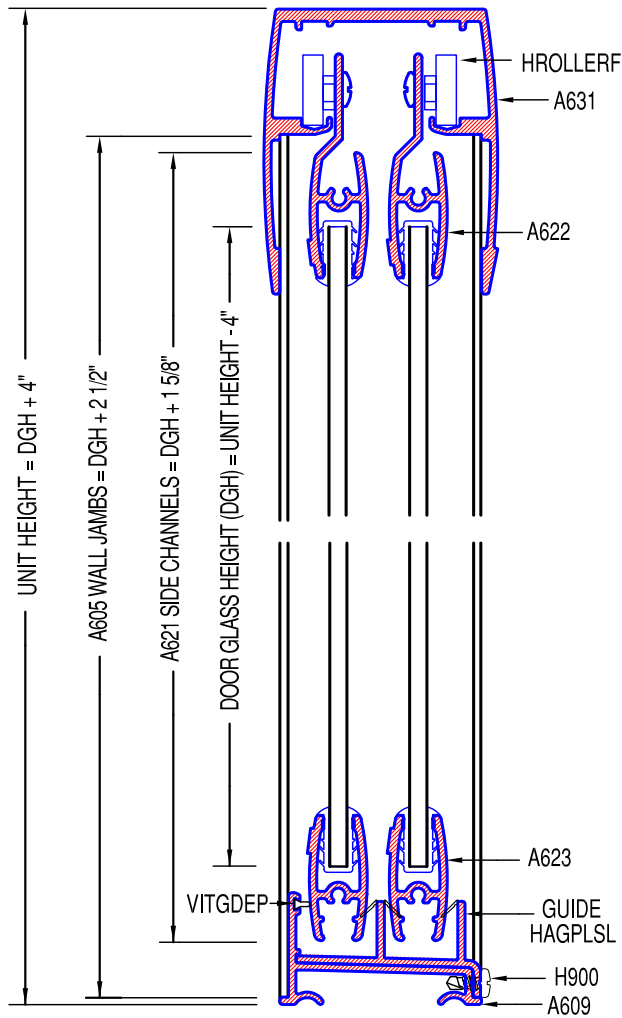
VERTICAL CROSS SECTION
