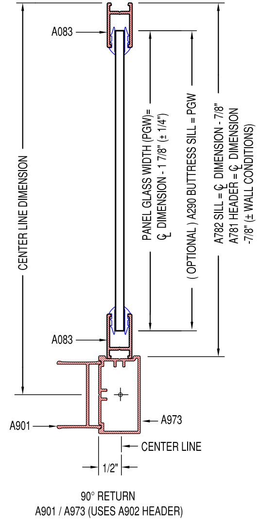
HORIZONTAL CROSS SECTION
