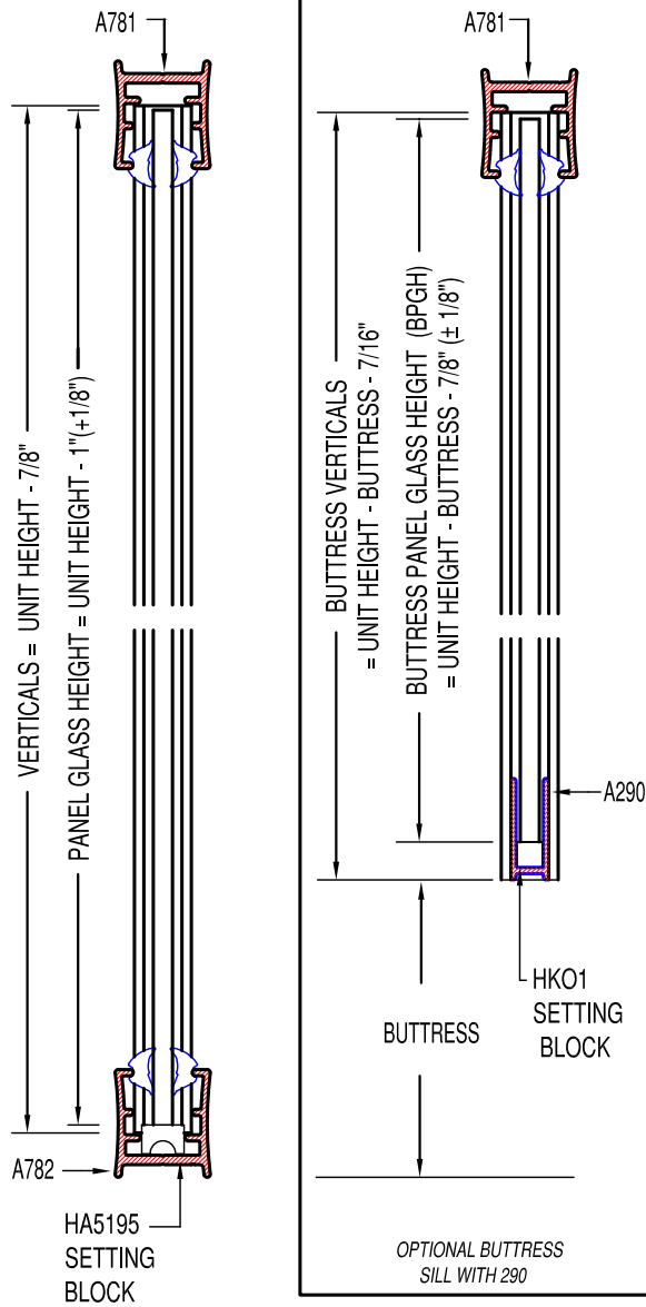
VERTICAL CROSS SECTION
