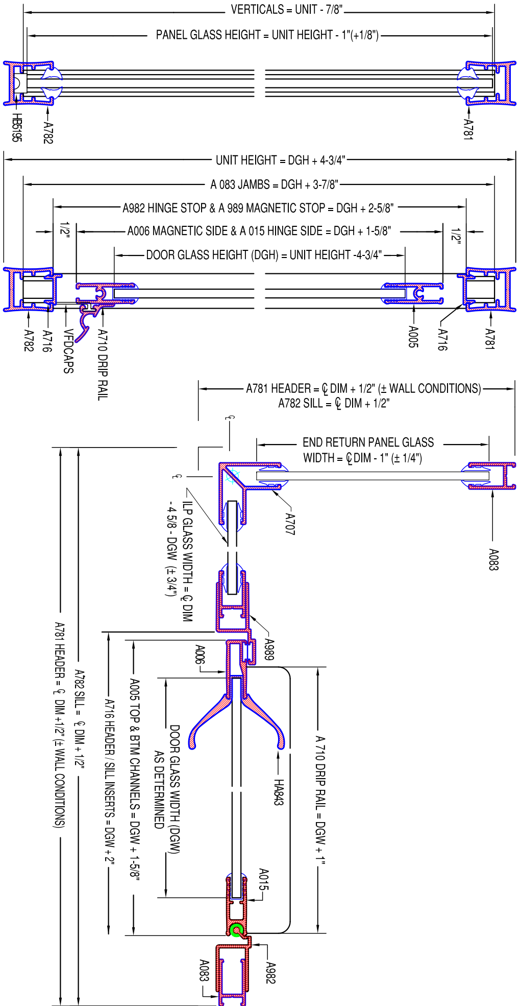
HORIZONTAL CROSS SECTION
