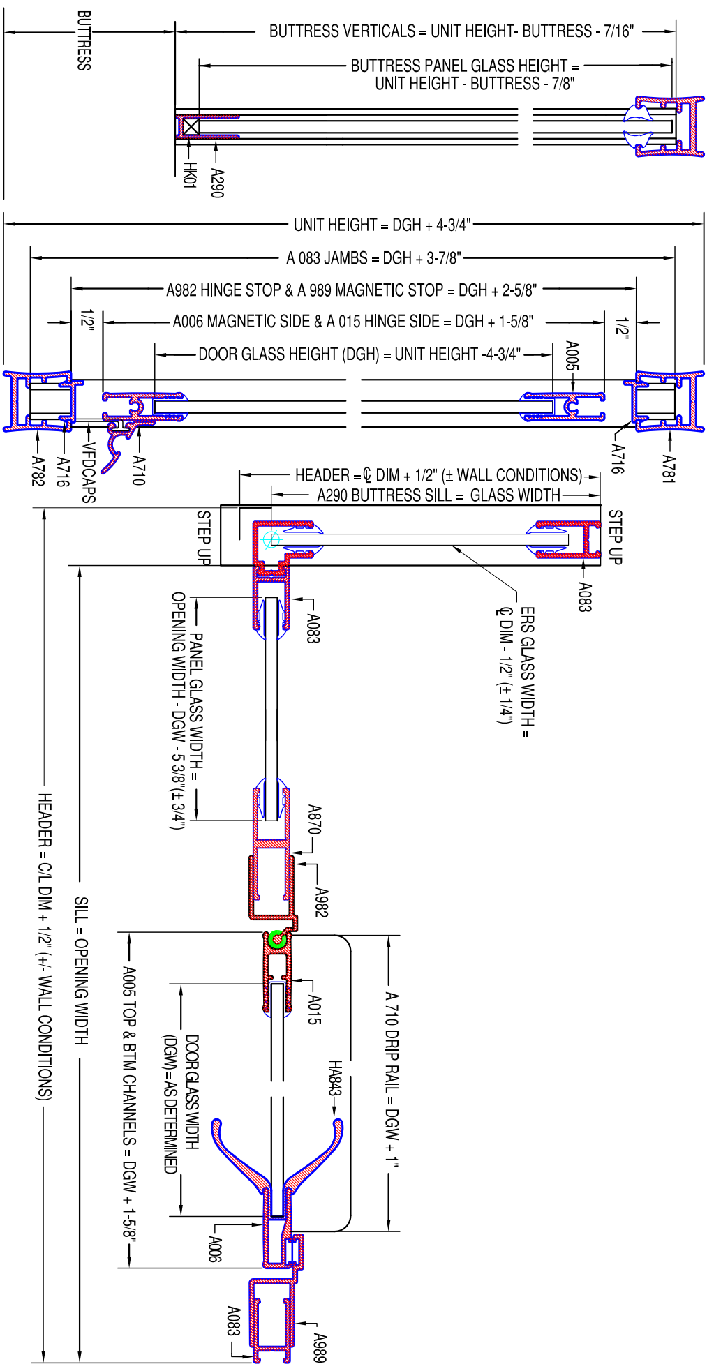
HORIZONTAL CROSS SECTION
