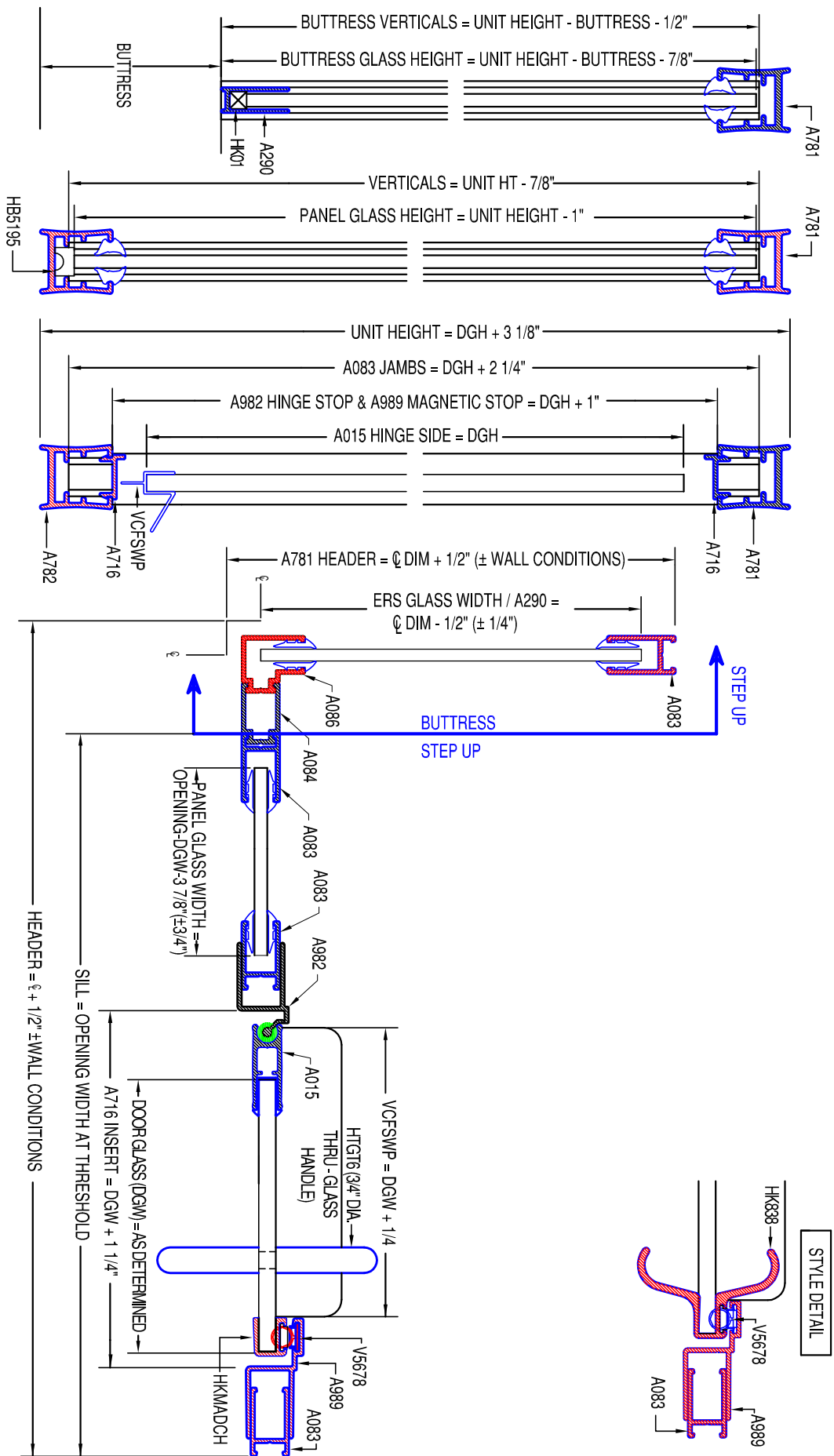
VERTICAL CROSS SECTION
