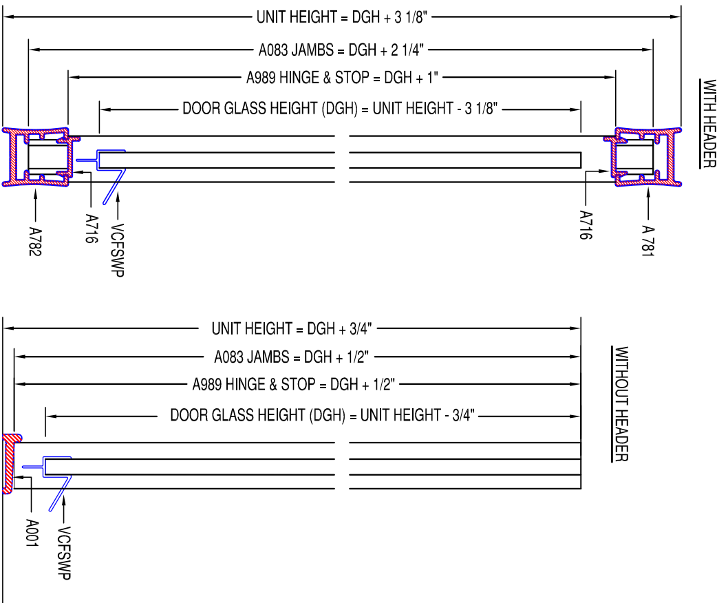
VERTICAL CROSS SECTION
