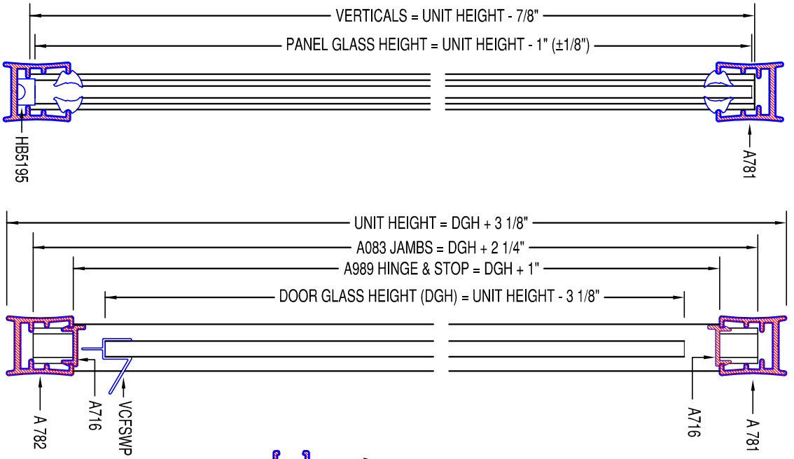
VERTICAL CROSS SECTION
