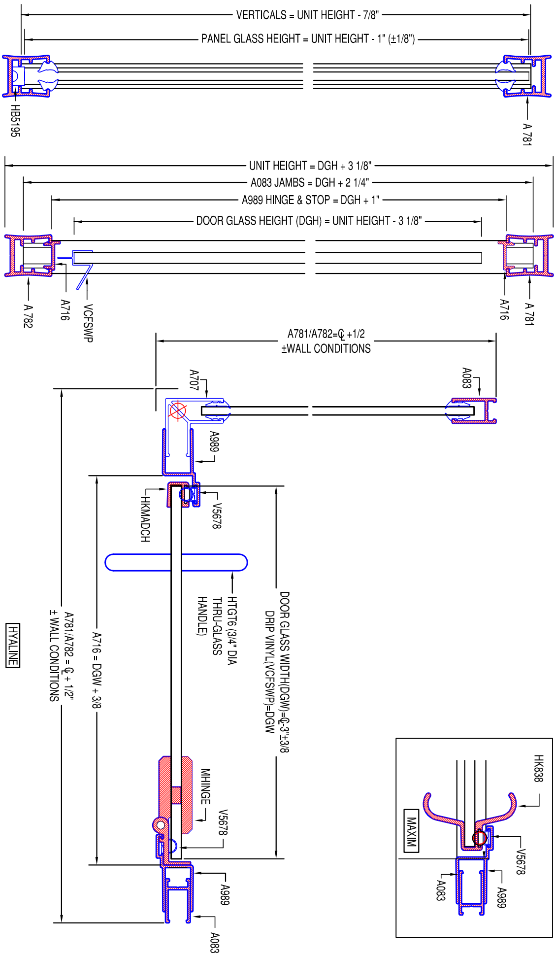
VERTICAL CROSS SECTION
